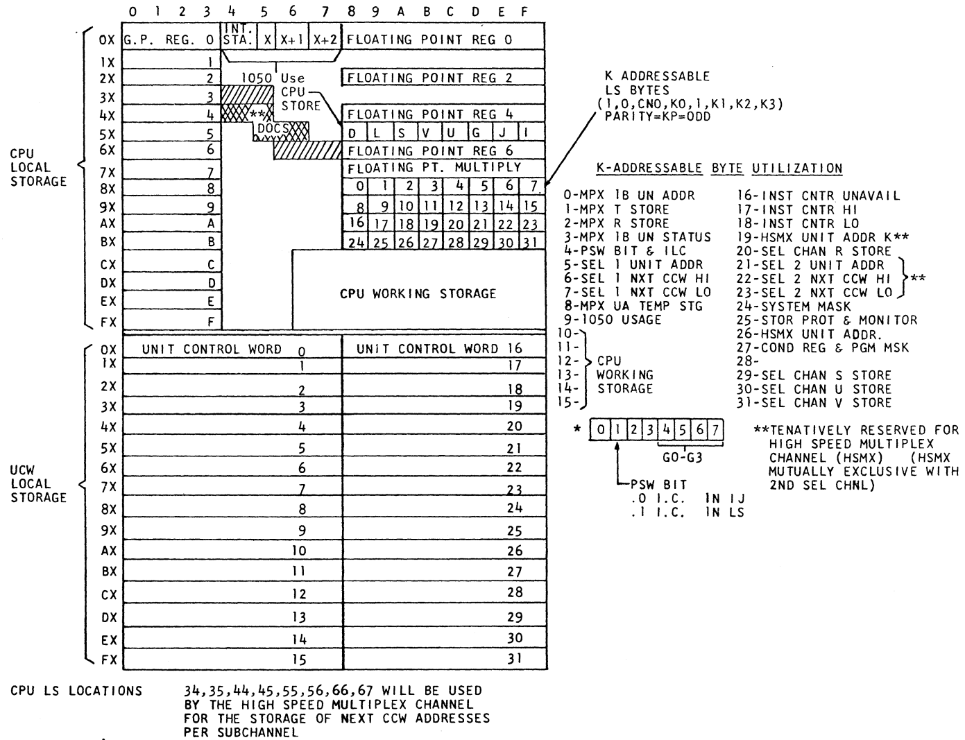
Figure A-4 2030 Local Storage Map
